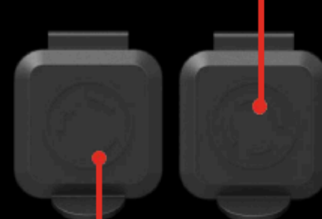
120V AC 30A L5-30R 120/240V AC 30A L14-30R
